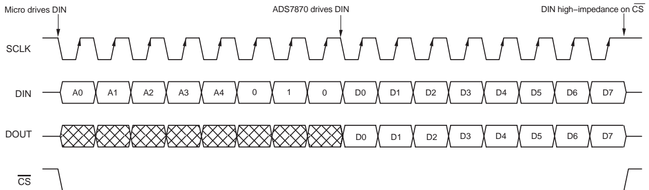
Figure 30. Timing for High Impedance State on DIN/DOUT ( \overline{CS} = 1 )
